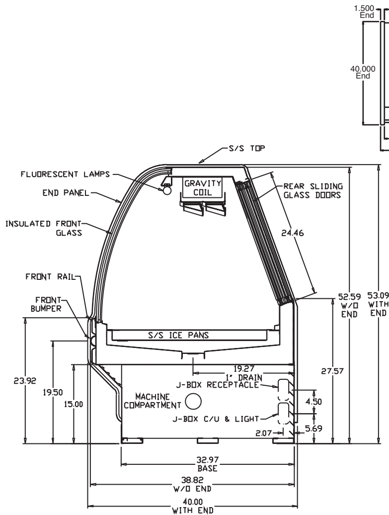
Cross Section
