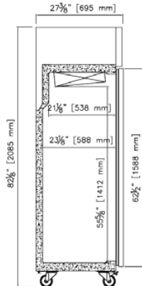
RIGHT VIEW
