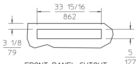
FRONT PANEL CUTOUT SINGLE CONTROL PANEL
