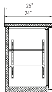
Side Section
