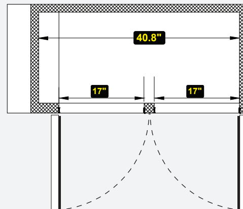
Top View Inside Cabinet
