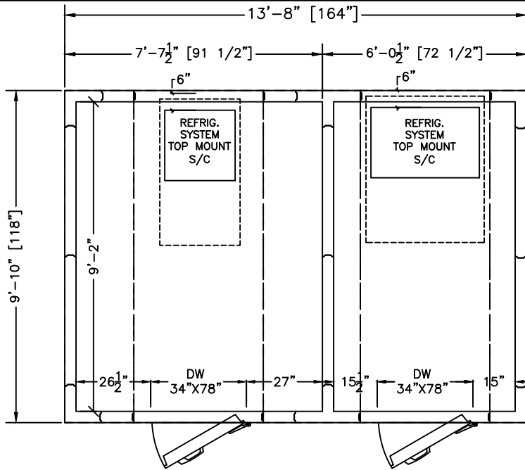
COOLER (NO FLOOR PANELS)
