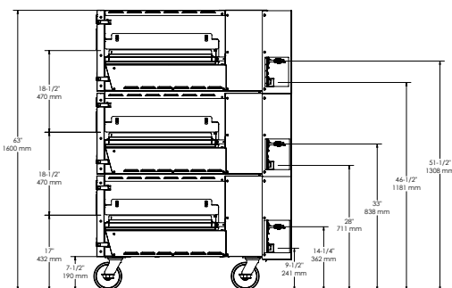
2824 Gas Triple Stack Side View
