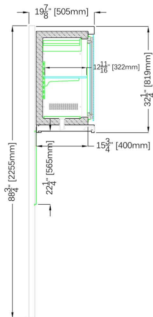
A - 19 7/8"D (505MM) 88 3/4"H (2255MM) WITH WALL PANEL
