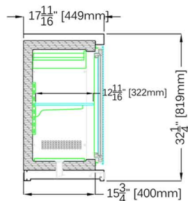
B - 17 11/16"D (449MM) 32 1/4"H (819MM) WITHOUT WALL PANEL
