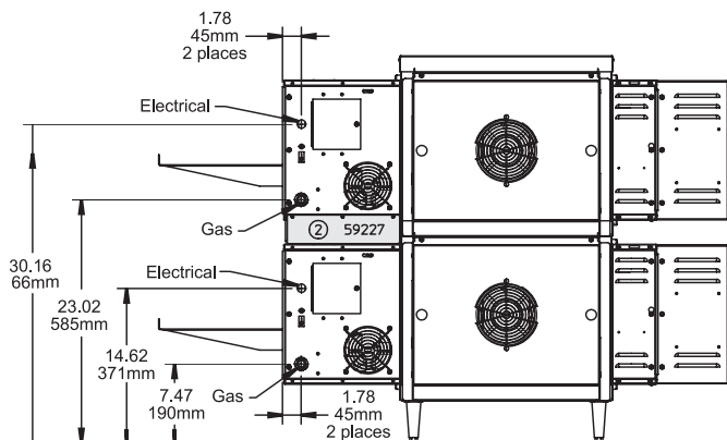
PS520 Back View – Gas, Double Stacked Units
