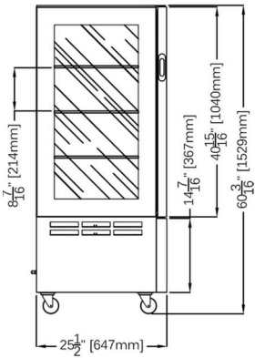
VC6314 H60 & VC8314 H60
